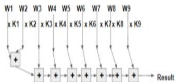
Fig.7 MAC
