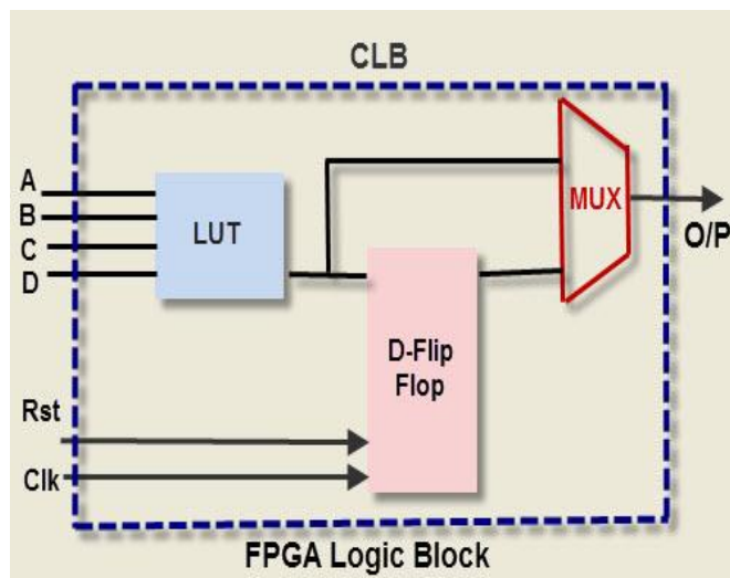
Fig.1 FPGA Block
